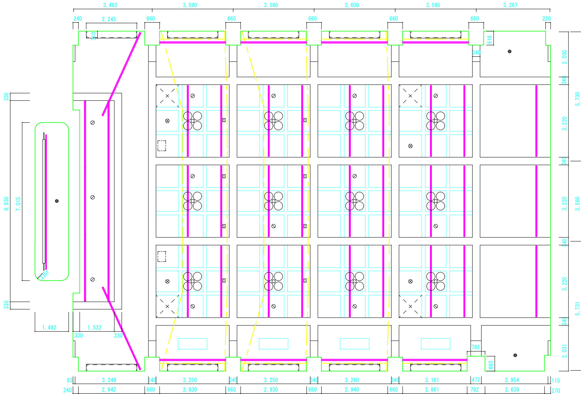
Kyoto Art Center 2F KOUDOU S=1/100
