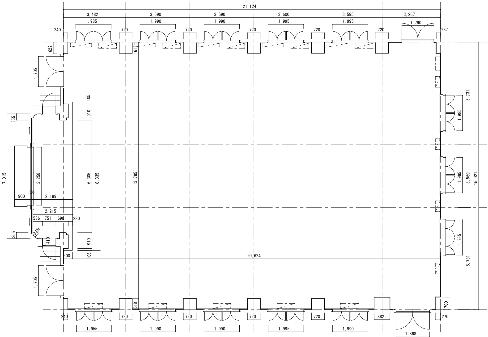
Kyoto Art Center 2F KOUDOU S=1/100
